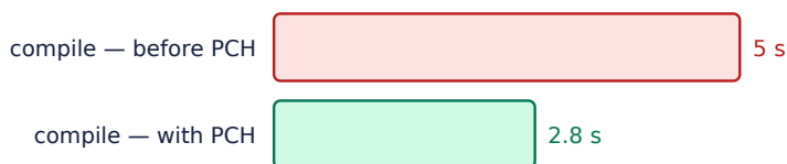
Fig 6.2 — precompiling <bits/stdc++.h> . Counter-intuitively, -O0 was slower than -O2 — the header parse dominates, not codegen.
